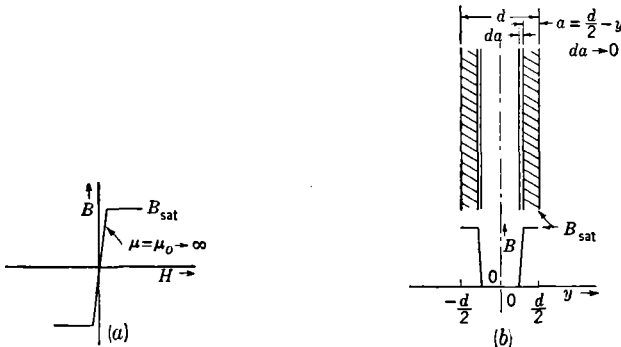
FIG. 15-23.—(a) Idealized B - H loop for a material of \mu = \mu_0 = \infty and H_c = 0 . (b) Instantaneous distribution of flux density within the lamination for nonlinear magnetization where \mu = \mu_0 = \infty and H_c = 0 .
